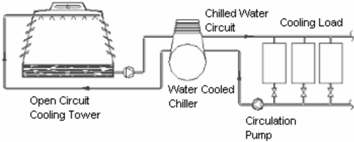
Water cooled chiller, open circuit cooling tower
