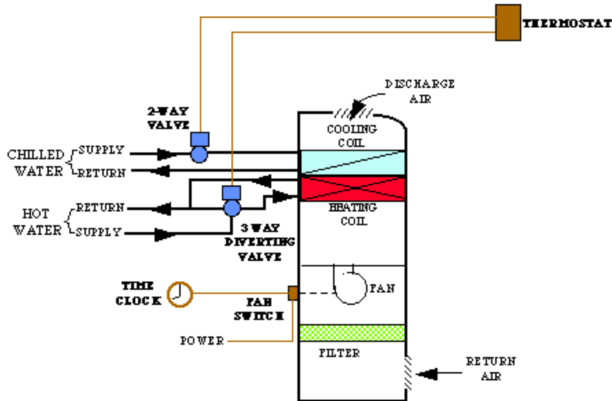
Fan-Coil Unit using 4-way piping for heating and cooling along with 2-way and 3-way diverter valve for temperature control
