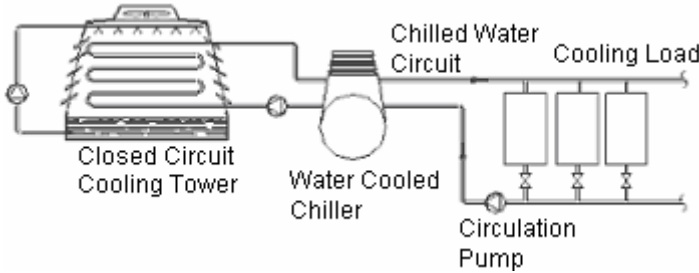
Water Cooled Chiller, Closed Circuit Cooling Tower
