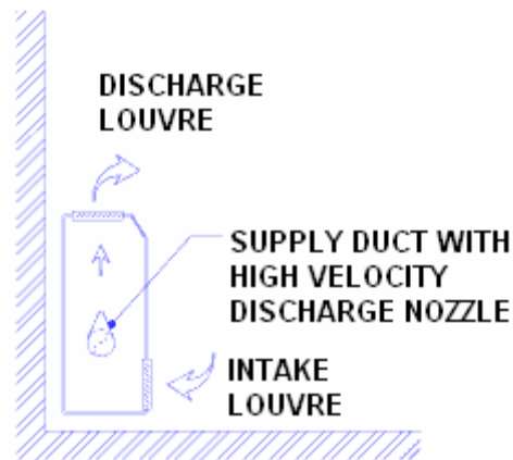
Induction unit
