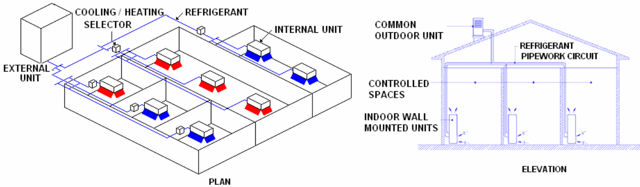
Variable Volume Refrigerant Units
