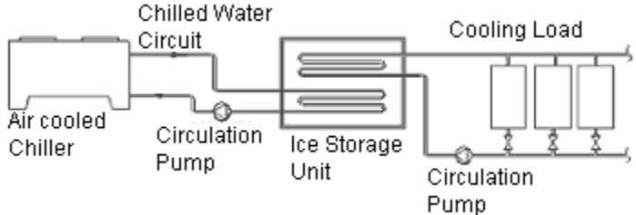
Air cooled chiller, ice storage option
