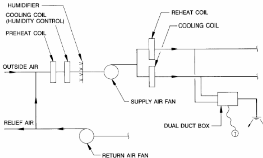
Dual Duct Constant Air Volume System
