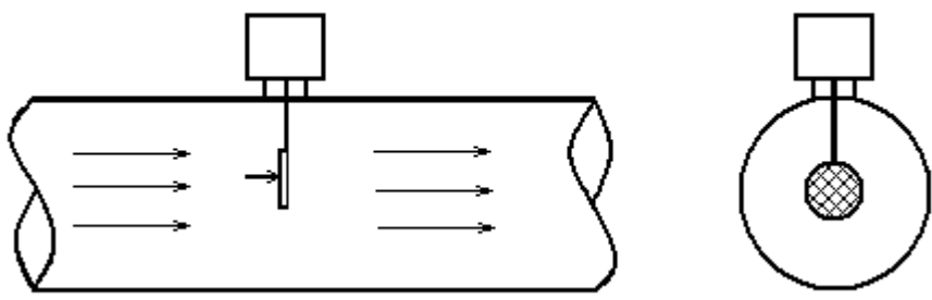
Figure 8. Target Flow Meter
