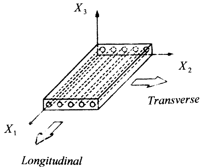
Figure 3.2. Natural (Material) Coordinates of Unidirectionally Reinforced Lamina
