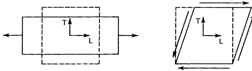
Figure 2.3. Extensional and Shear Deformation, Orthotropic Material, (Loaded Along Material Coordinates)
