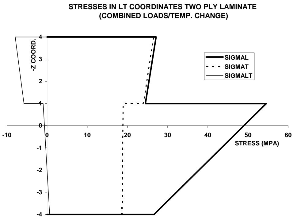
Figure 7.11 Stress Variation for [45/0] Laminate, Natural Coords., Combined Loads
