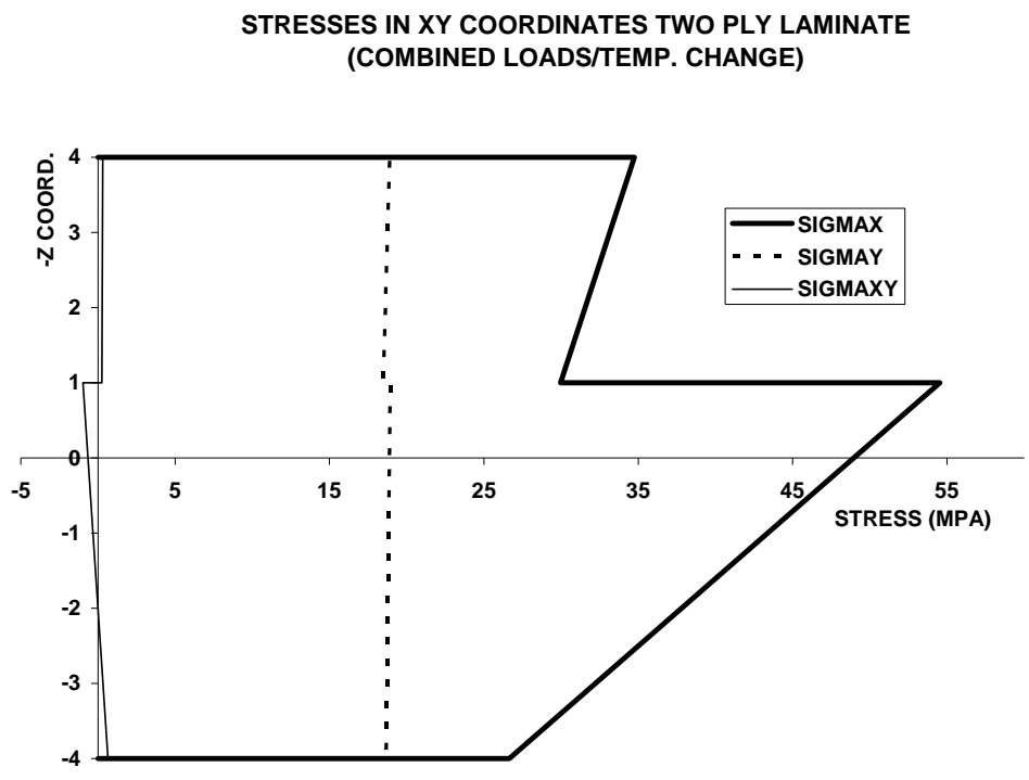
Figure 7.10 Stress Variation for [45/0] Laminate, Ref. Coords., Combined Loads
